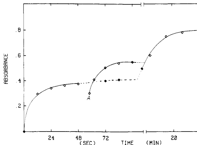
Figure 4. Absorbance at 400 nm vs time for the cleavage of benzoate and the appearance of p -nitrophenylate from sonicated covescicular 7/5 under the flip-flop protocol described in the text; see Table IV. The dotted line refers to a control experiment in which the heating step was omitted. 30 The reduced absorbance at point A is discussed in the text.
